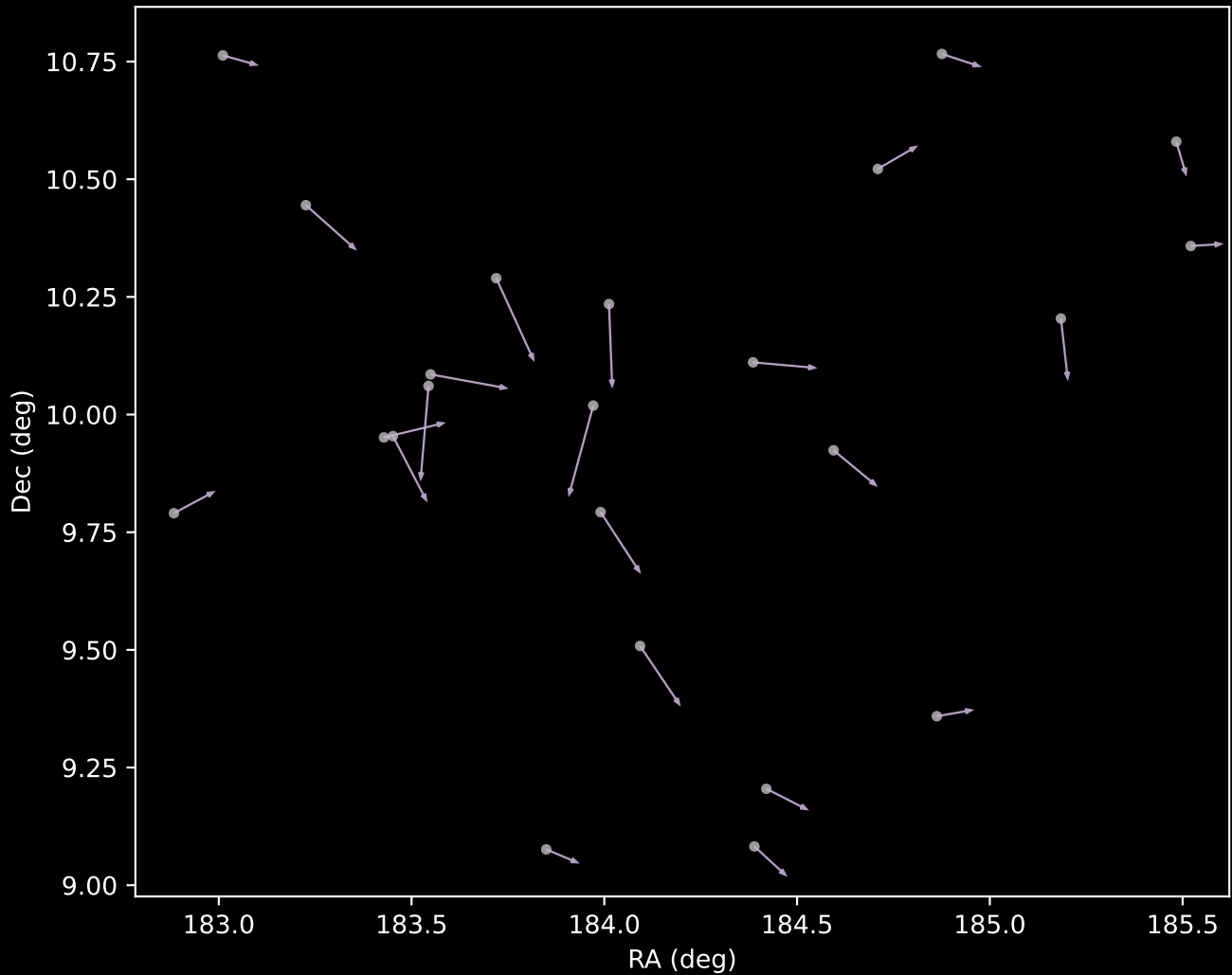
APOGEE DR17 Cluster 9 Proper Motion Vectors (n=23)
