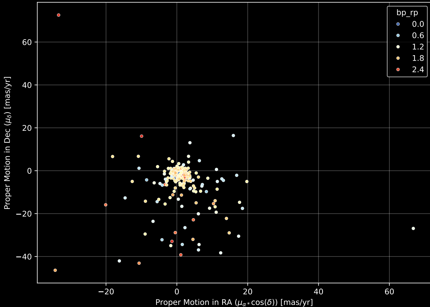
APOGEE DR17 Field: [LAMBDAORI-A] Proper Motion Diagram (n= 398)
