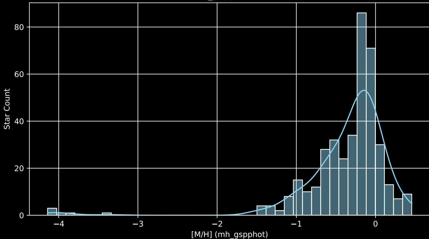
APOGEE DR17 Field: [LAMBDAORI-A [M/H] (mh_gspphot) (n= 395)
