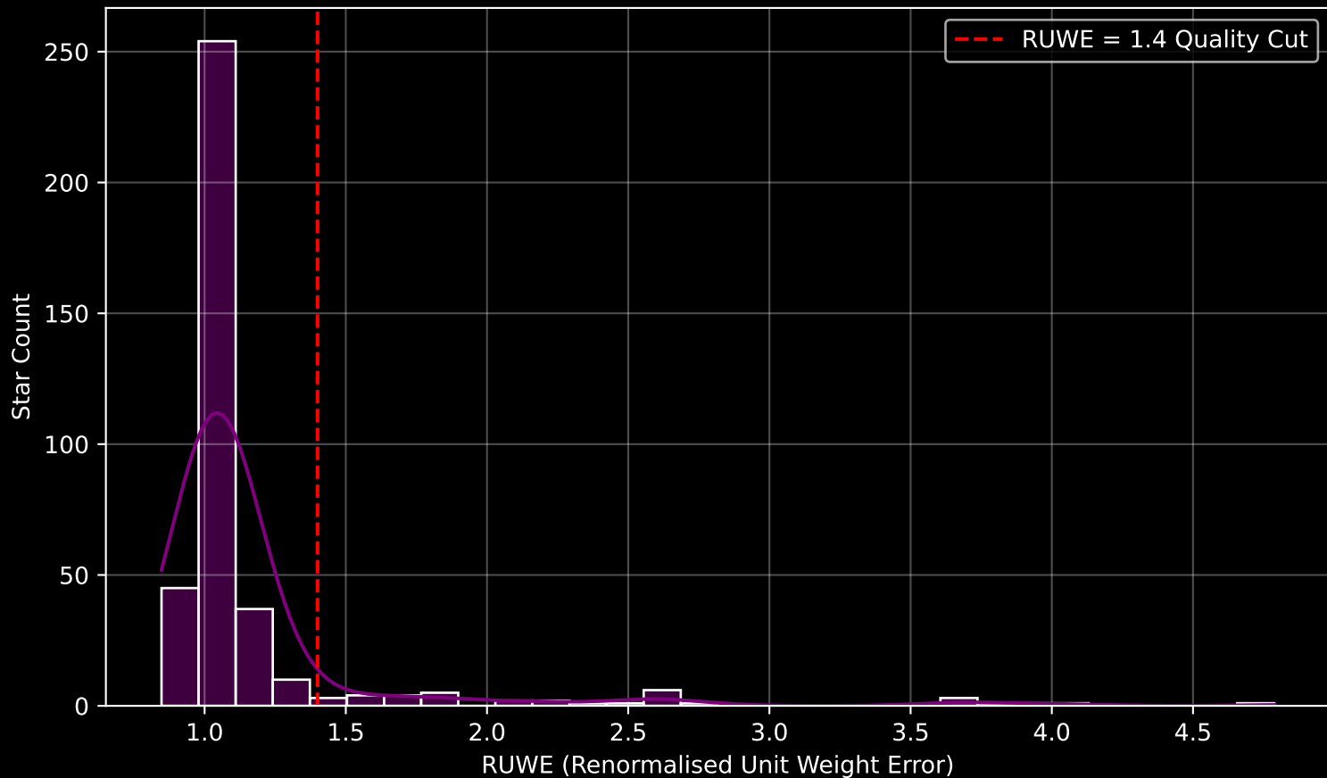
GAPOGEE DR17 Field [LAMBDAORI-A] RUWE Distribution (n= 382)
