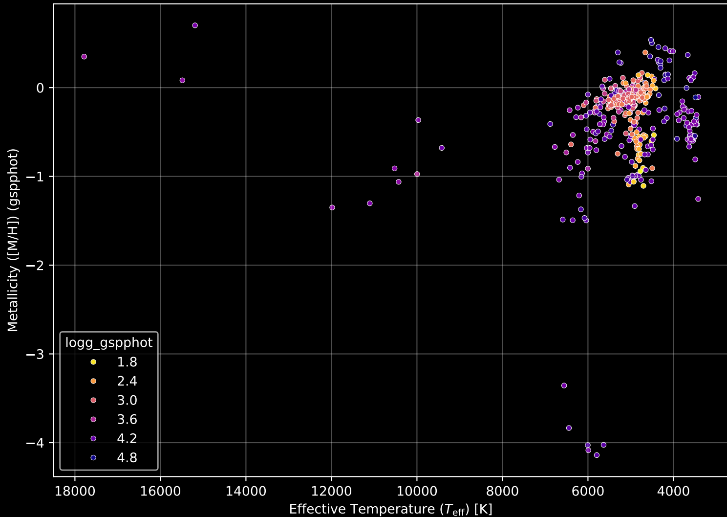
APOGEE DR17 Field: [LAMBDAORI-A] Stellar Population Parameters (n= 398)
