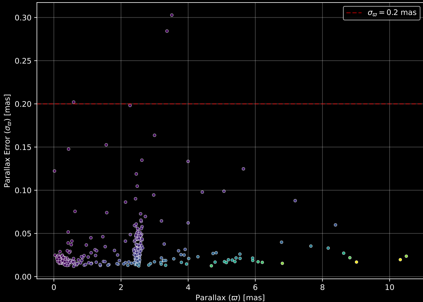
APOGEE DR17 Field: [LAMBDAORI-A] Parallax Quality (n= 398)
