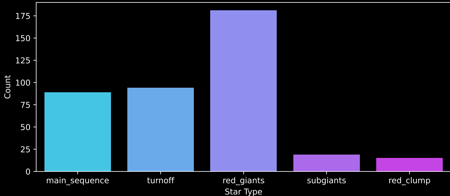
APOGEE DR17 Field: [LAMBD AORI-A] Count plot of Star Type
