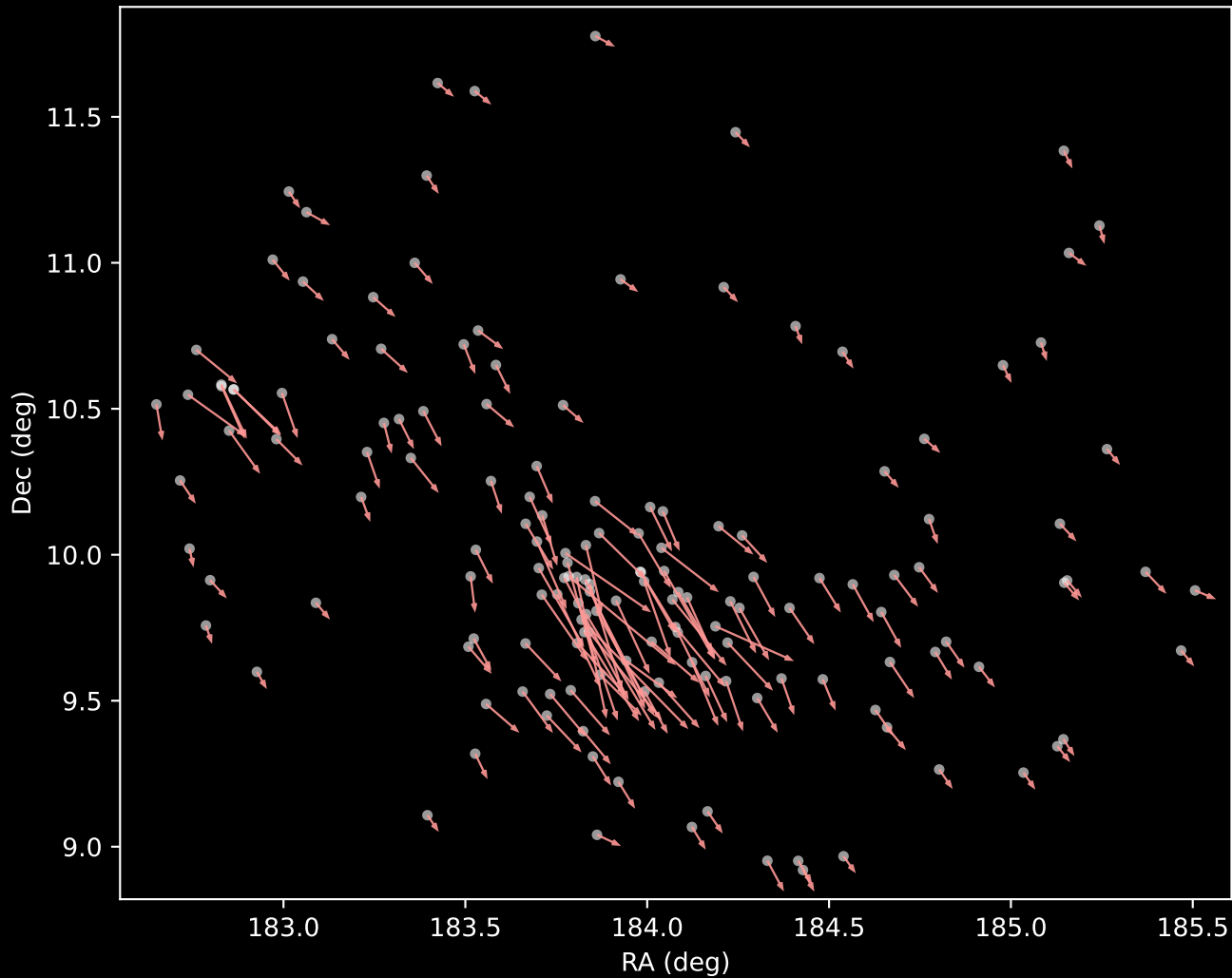
APOGEE DR17 Cluster 7 Proper Motion Vectors (n=156)
